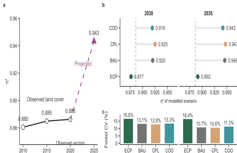
Fig. 3. Multi-temporal variance decomposition ( \eta^2 ) of InVEST HQ. (a) Observed land cover for 2010, 2015, 2020 ( \eta^2 = 0.880, 0.885, 0.886 ; n = 31,889 per year) and projected 2025 ( \eta^2 = 0.943 ). No confidence bands are shown because each year is a single model output. (b, c) Four modelled scenarios (ECP, BAU, CPL, COO) at 2030 and 2035: scenario \eta^2 (b) and forest within-class CV (c). Baseline 2020 observed \eta^2 = 0.886 . Scenarios are policy-sensitivity explorations, not winner identification.
