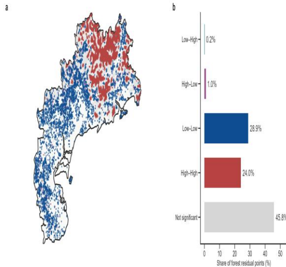
Fig. 4. Local Moran's I (LISA) clusters of forest within-class HQ residuals (2020; n = 15,440 forest sampling points; KNN k = 8 ; 999 permutations; p < 0.05 ). Global Moran's I = 0.752 . (a) LISA cluster map. (b) Cluster shares: high-high 24.0%, low-low 28.9%, high-low 1.0%, low-high 0.2%, non-significant 45.8%.
