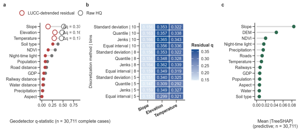
Fig. 6. Driver attribution of HQ variance and sensitivity to land-cover detrending. (a) Paired raw-to-residual Geodetector q-statistics for 13 factors ( n = 30,711 complete cases) before and after LUCC detrending; top-3 attenuation \Delta q : Slope 0.370, Elevation 0.167, Temperature 0.172. (b) Residual-q sensitivity across four discretization methods (quantile, equal-interval, Jenks, standard-deviation) \times three bin counts (5, 8, 10) for the three leading factors. (c) Mean |TreeSHAP| from the XGBoost model of HQ on thirteen exogenous factors (five-fold CV R^2 = 0.683 ); a predictive-attribution artifact, not a causal statement. The spatial-share attribution output is excluded because its denominator could not be reconciled with the stored artifact.
