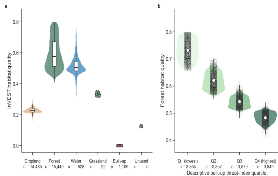
Fig. 2. Per-class distribution of InVEST habitat quality (HQ, 2020, 1-km grid) and descriptive forest stratification. (a) Raincloud/violin + raw-point distributions of HQ for six land-cover classes ( n = 31,889 ; forest n = 15,440 , cropland n = 14,485 , water n = 828 , built-up n = 1,109 , grassland n = 22 , unused n = 5 ). (b) Forest HQ by descriptive quartile of built-up threat-index exposure (identical H_j = 0.80 ; n = 15,440 ; Q1 n = 3,864 , mean = 0.732; Q2 n = 3,857 , mean = 0.621; Q3 n = 3,870 , mean = 0.542; Q4 n = 3,849 , mean = 0.483). Quartile comparisons are descriptive associations of spatial configuration, not fitted causal effects.
