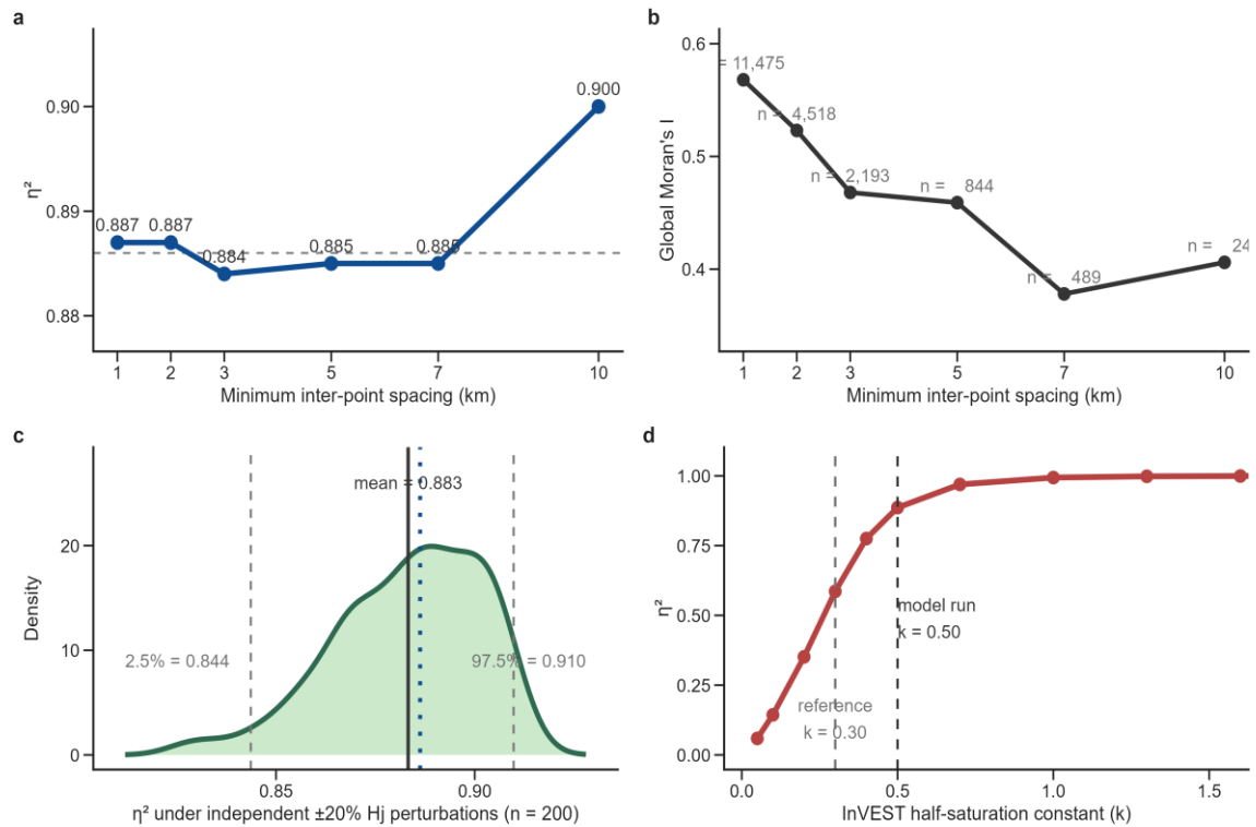
Fig. 5. Sensitivity diagnostics of the variance decomposition. (a) \eta^2 across greedy spatial thinning (1–10 km minimum inter-point spacing); \eta^2 remained within 0.884–0.900. (b) Global Moran's I of HQ declined from the full-set value 0.615 to 0.406 at 10 km (first thinned spacing 1 km = 0.568); thinning values originate from the manuscript's Table 10 (n = 241–11,475 retained), whose historical producer has not been independently reproduced. (c) \eta^2 under independent \pm 20\% H_j perturbations (n = 200
