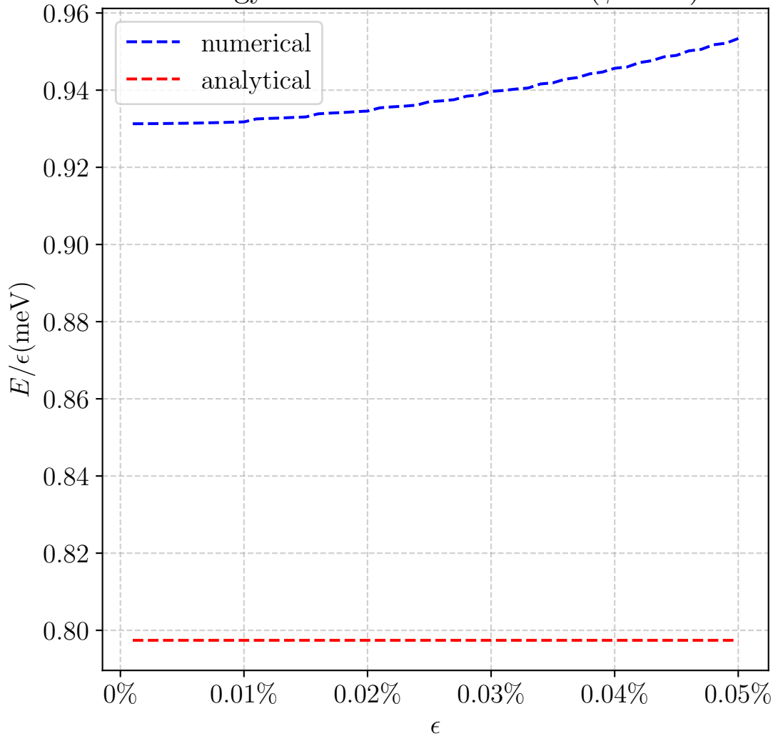
Energy of Shifted Dirac Points( \phi = 0^\circ )
