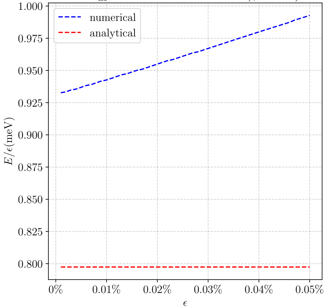
Energy of Shifted Dirac Points( \phi = 10^\circ )
