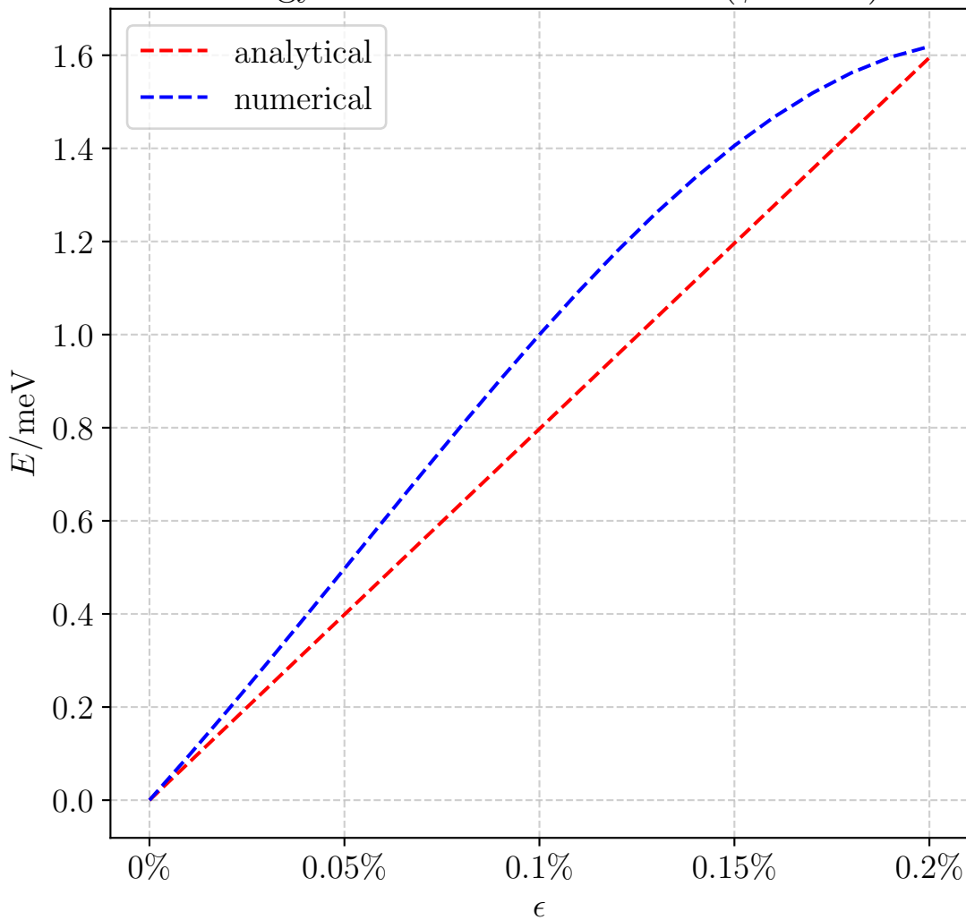
Energy of Shifted Dirac Points( \phi = 20^\circ )
