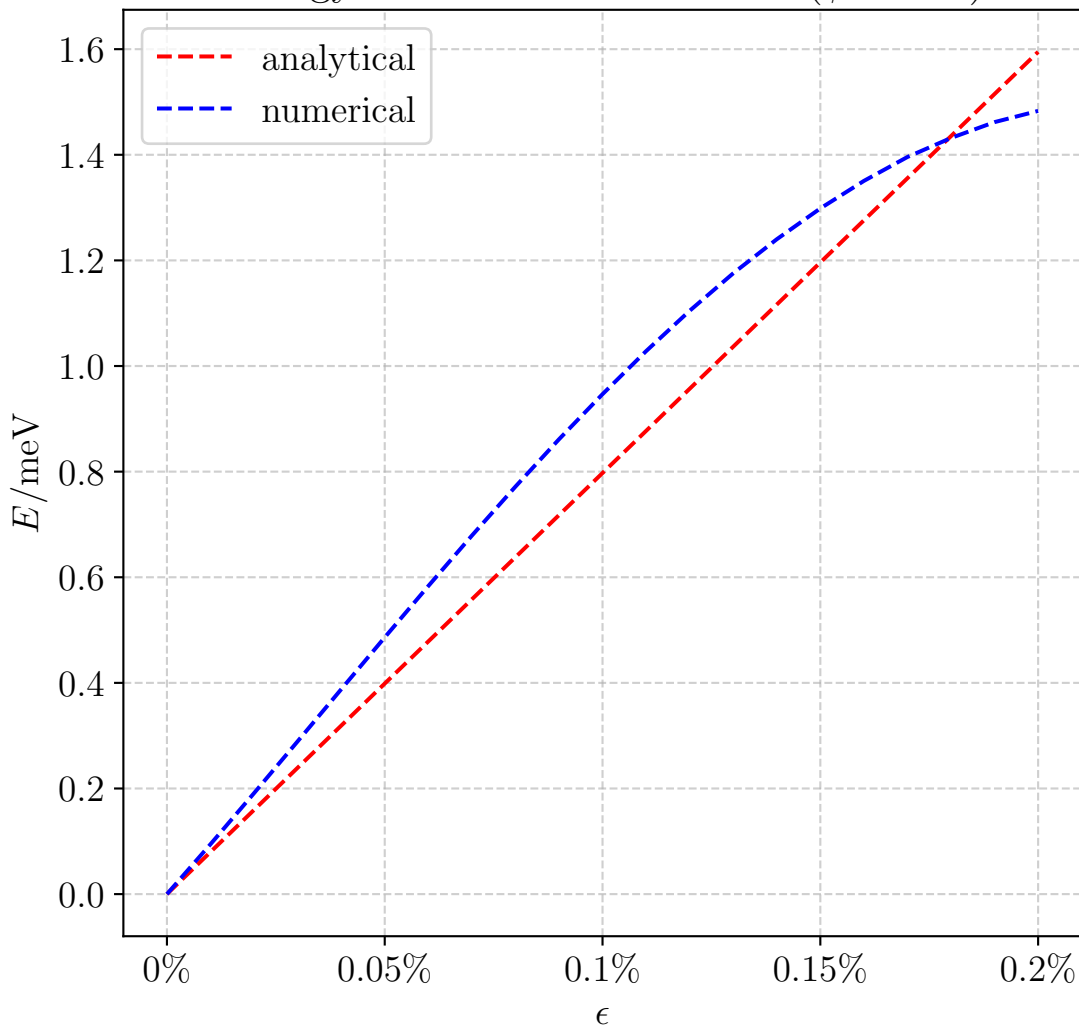
Energy of Shifted Dirac Points( \phi = 30^\circ )
