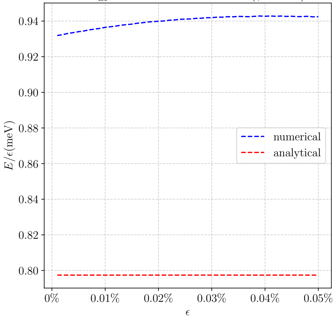
Energy of Shifted Dirac Points( \phi = 40^\circ )
