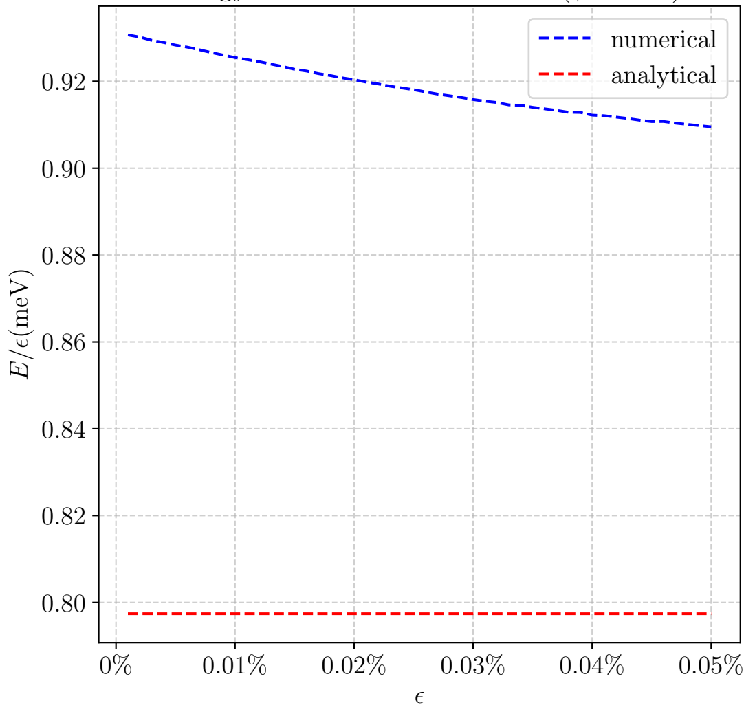
Energy of Shifted Dirac Points( \phi = 50^\circ )
