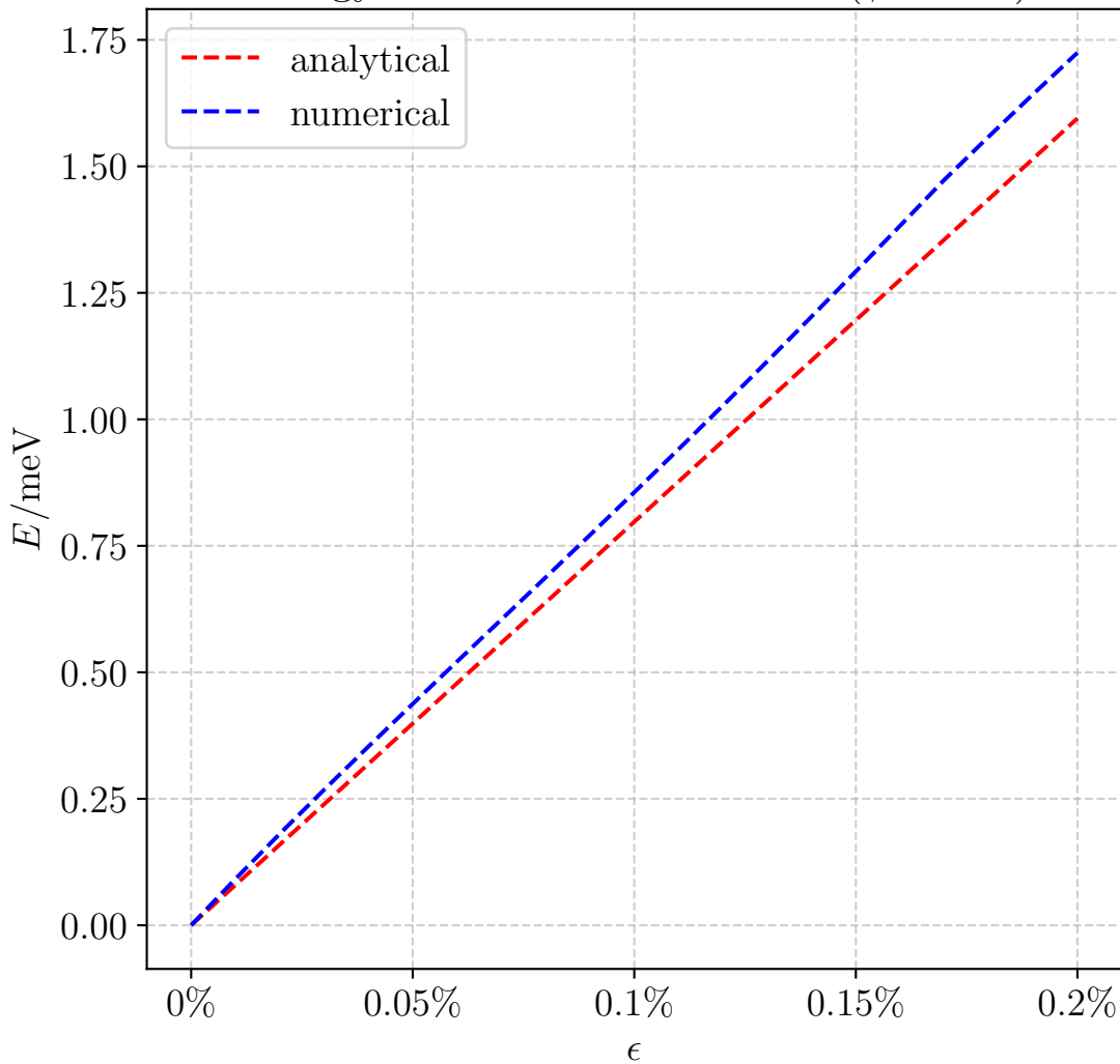
Energy of Shifted Dirac Points( \phi = 60^\circ )
