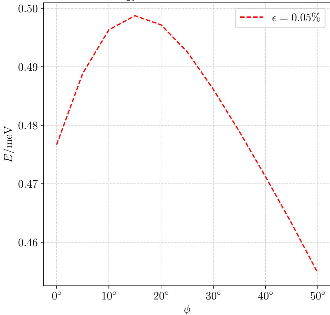
Energy of Shifted Dirac Points
