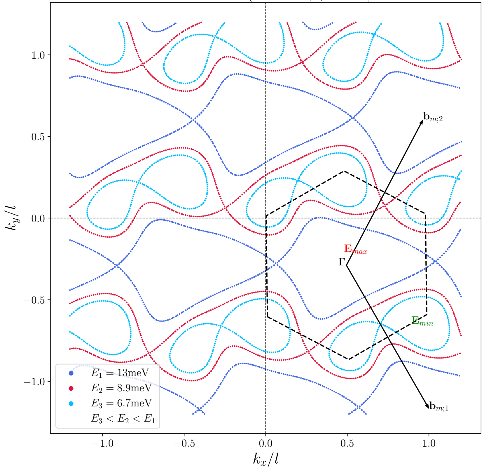
Fermi surface ( \epsilon = 0.1\% , \phi = 40^\circ )
