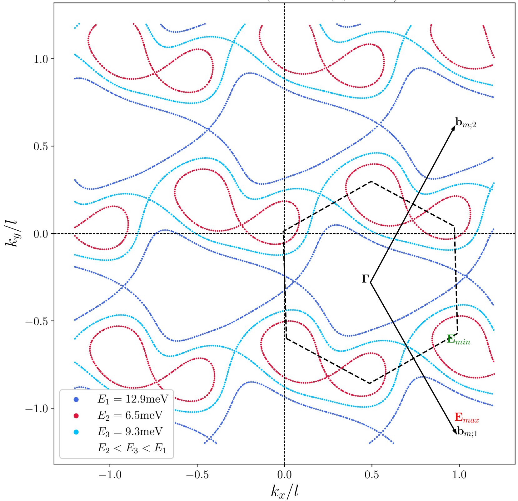
Fermi surface ( \epsilon = 0.1\% , \phi = 60^\circ )
