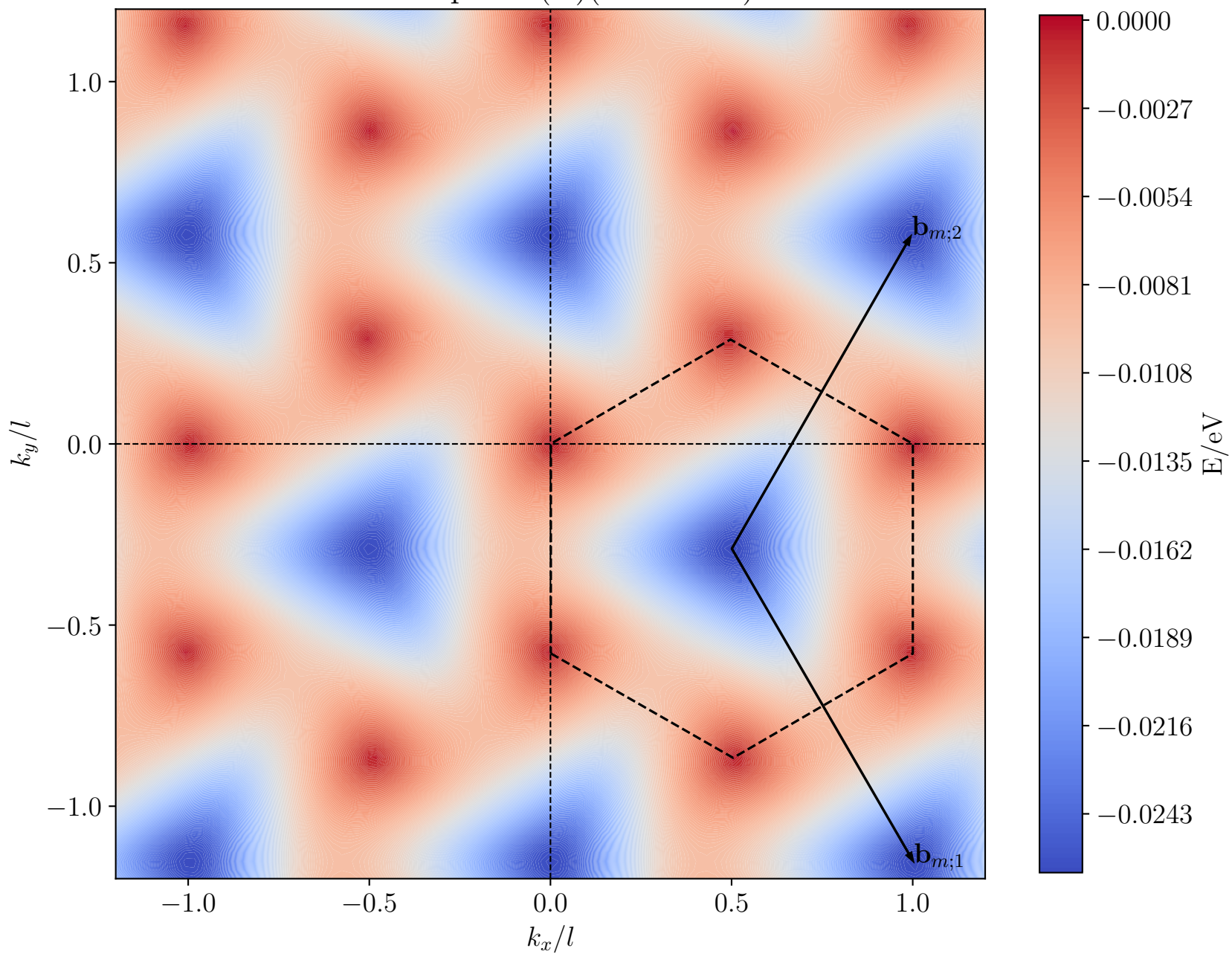
heatmap of E(N)(\epsilon = 0.01\%)
