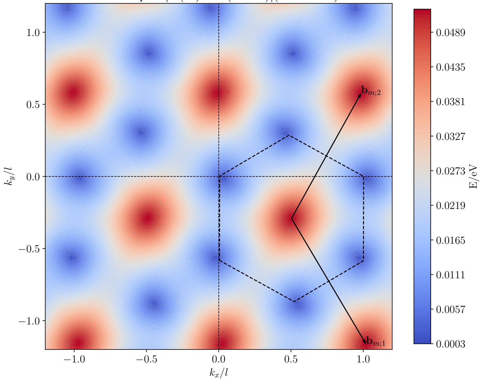
heatmap of |E(N) - E(N + 1)|(\epsilon = 0.05\%)
