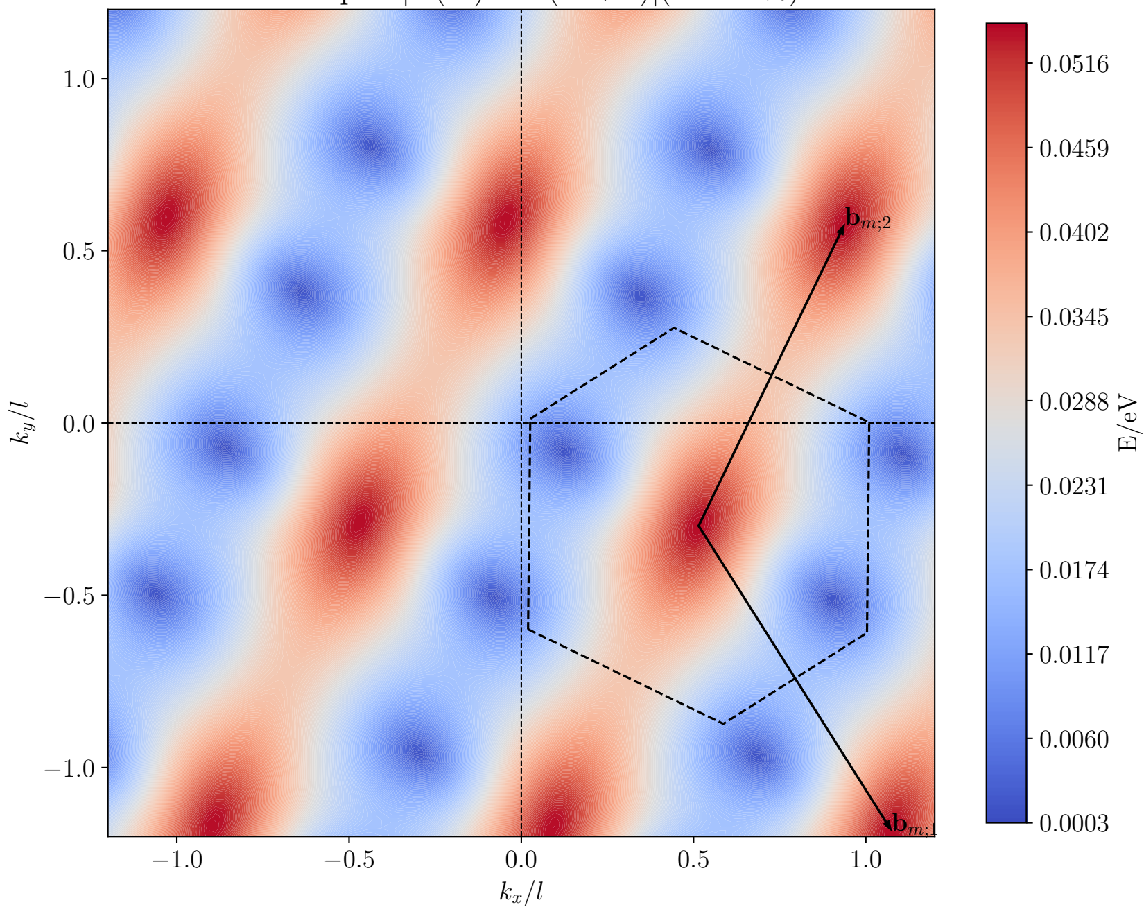
heatmap of |E(N) - E(N + 1)|(\epsilon = 0.2\%)
