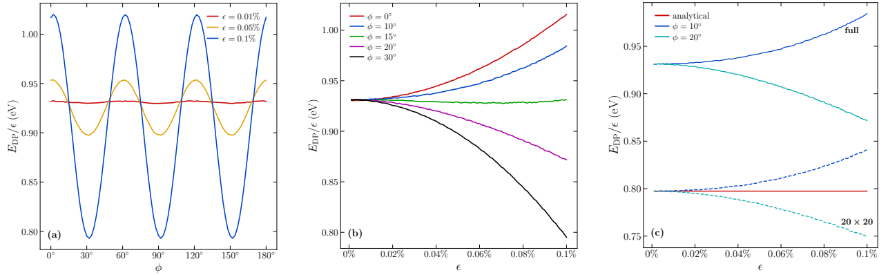
Figure 5: Ratio E_{DP}/\epsilon as a function of heterostrain parameters. (a) Dependence on the strain direction \phi for fixed \epsilon . (b) Dependence on the strain magnitude \epsilon for fixed \phi . (c) Comparison between the analytical perturbative result, the full numerical calculation, and the 20 \times 20 truncated-basis calculation. In (c), solid and dashed curves denote the full and 20 \times 20 numerical results, respectively.
