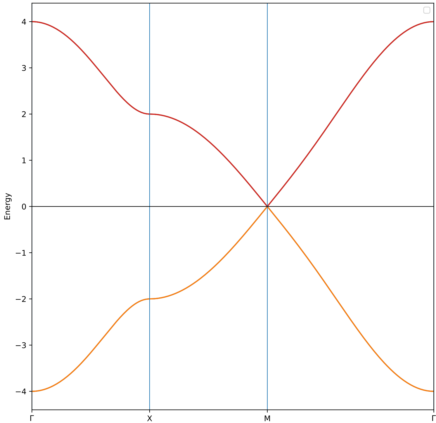
Bilayer QWZ band structure ( m = 2.0 , t_{\perp} = 0.0 , \lambda = 0.000 )
