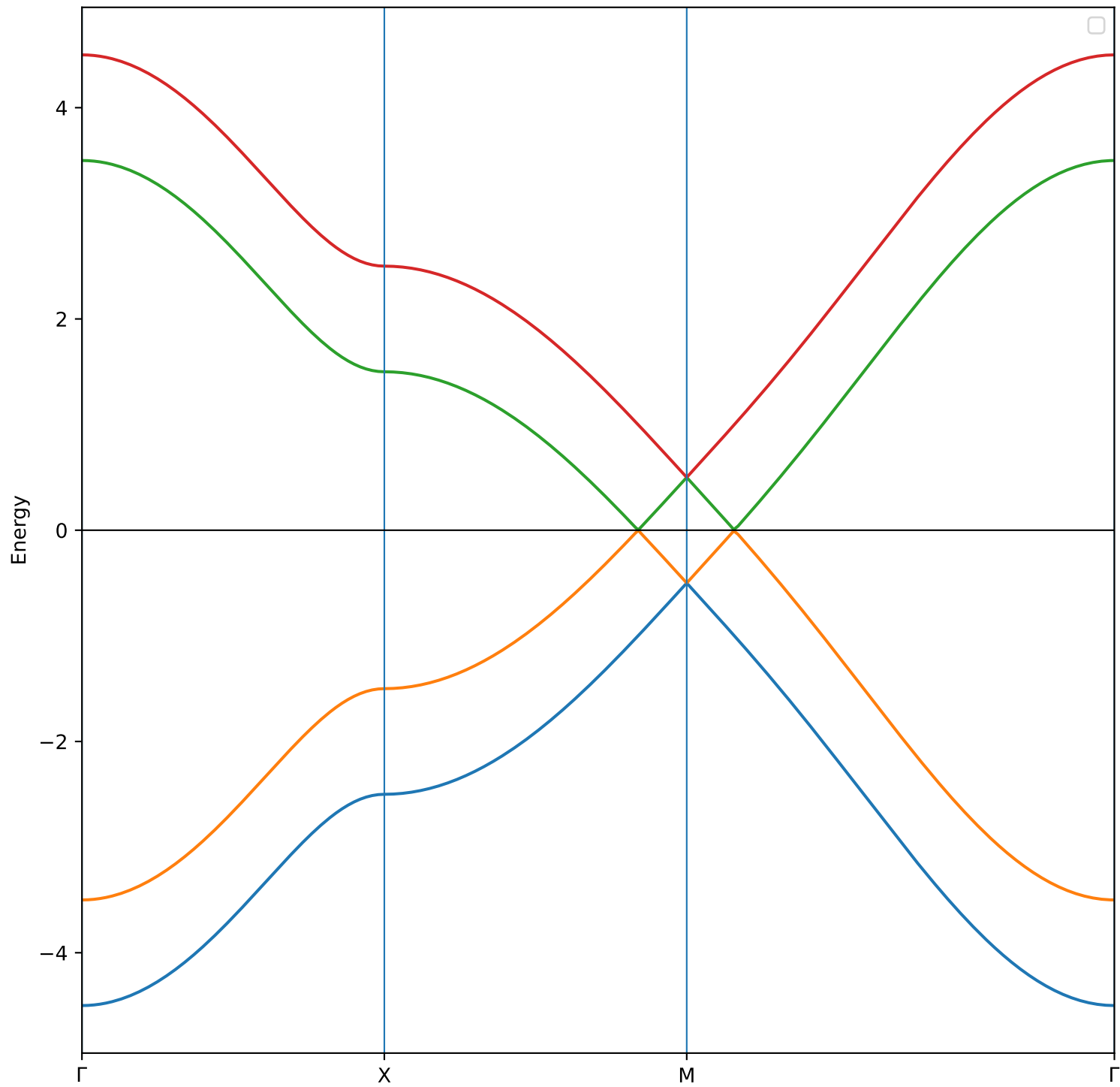
Bilayer QWZ band structure ( m = 2.0 , t_{\perp} = 0.5 , \lambda = 0.000 )
