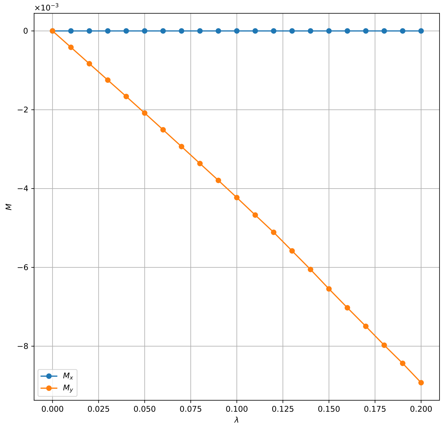
Bilayer QWZ Orbital Magnetization ( m = 1.0 , t_{\perp} = 0.2 , \mu = -1.0 , \delta = 1.00e-03 , N_k = 101 )
