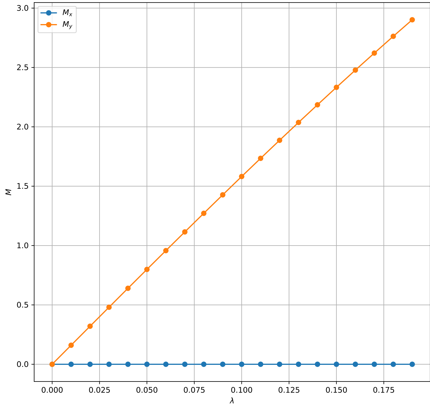
Bilayer QWZ Orbital Magnetization ( m = 1.0 , t_{\perp} = 0.2 , \mu = 0.0 , d = 1.0 )
