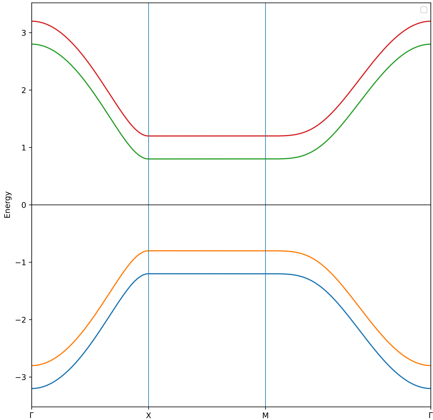
Bilayer QWZ band structure ( m = 1.0 , t_{\perp} = 0.2 , \lambda = 0.000 )
