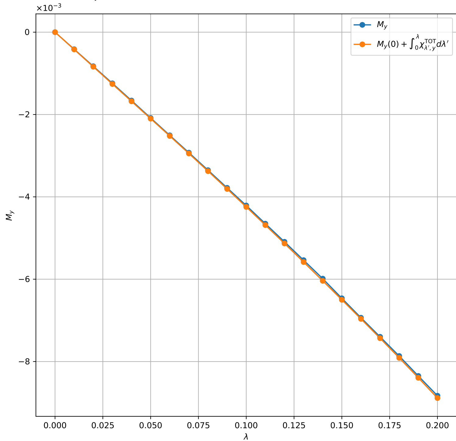
Bilayer QWZ: M_y vs. integrated susceptibility ( m = 1.0 , t_{\perp} = 0.2 , \mu = -1.0 , \eta = 0.03 , N_k = 251 )
