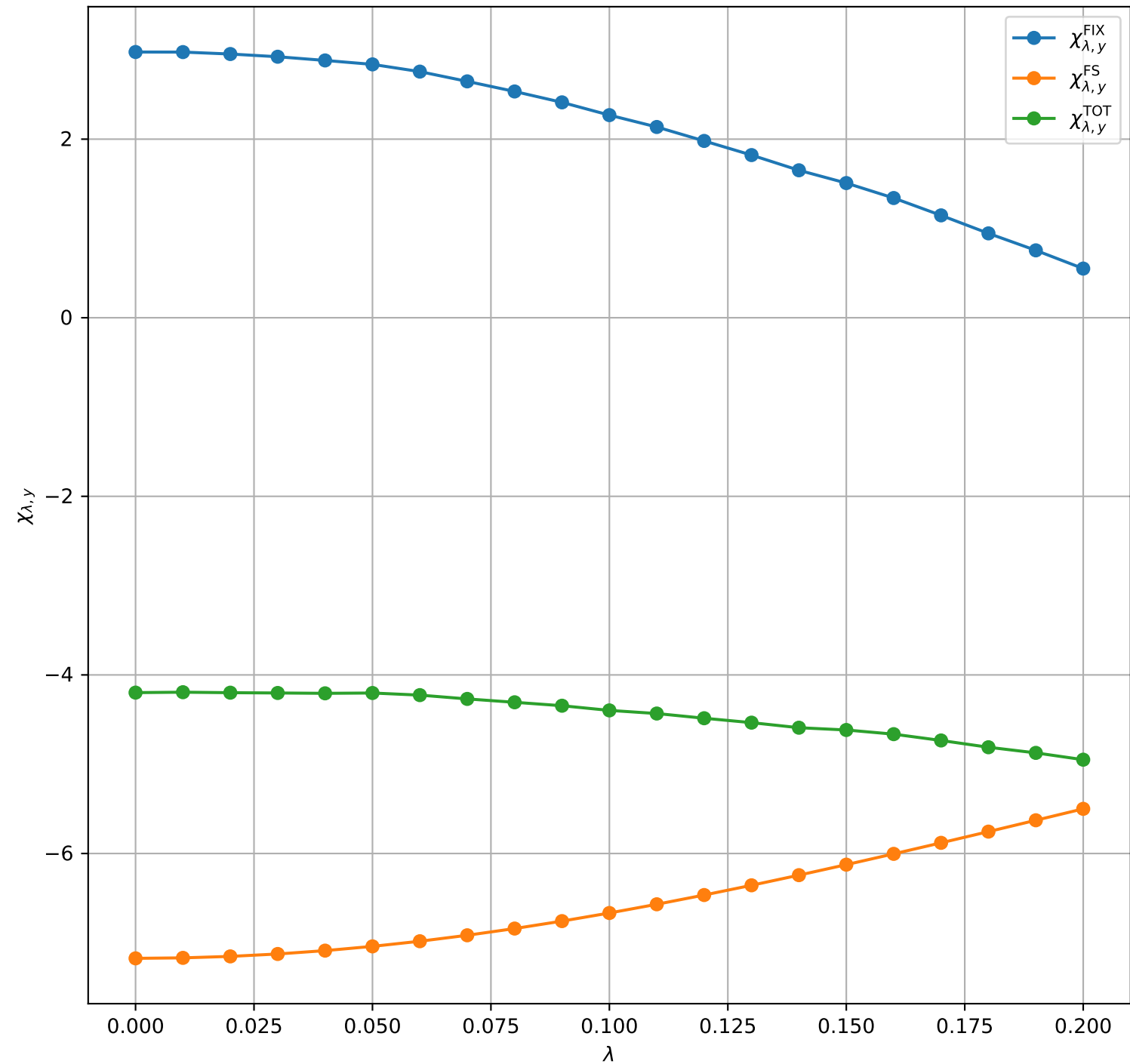
\times 10^{-2} Bilayer QWZ Susceptibility ( m = 1.0 , t_{\perp} = 0.2 , \mu = -1.0 , \eta = 0.03 , N_k = 251 )
