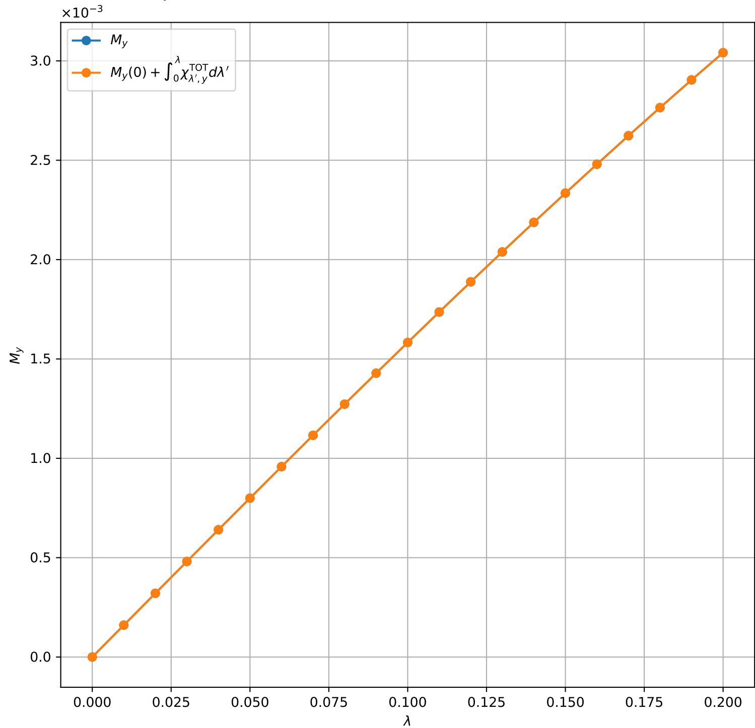
Bilayer QWZ: M_y vs. integrated susceptibility ( m = 1.0 , t_{\perp} = 0.2 , \mu = 0.0 , \eta = 0.03 , N_k = 251 )
