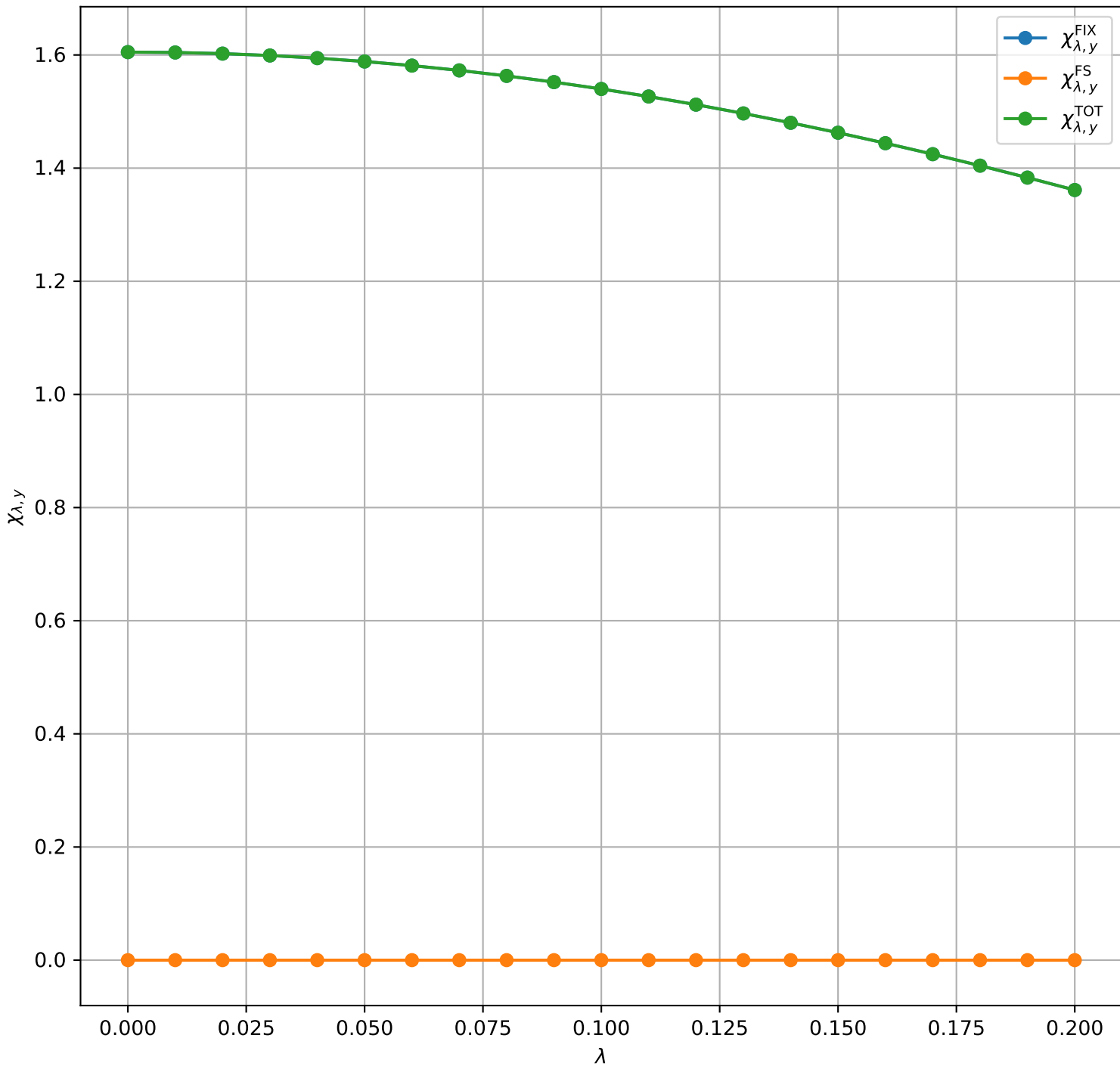
\times 10^{-2} Bilayer QWZ Susceptibility ( m = 1.0 , t_{\perp} = 0.2 , \mu = 0.0 , \eta = 0.03 , N_k = 251 )
