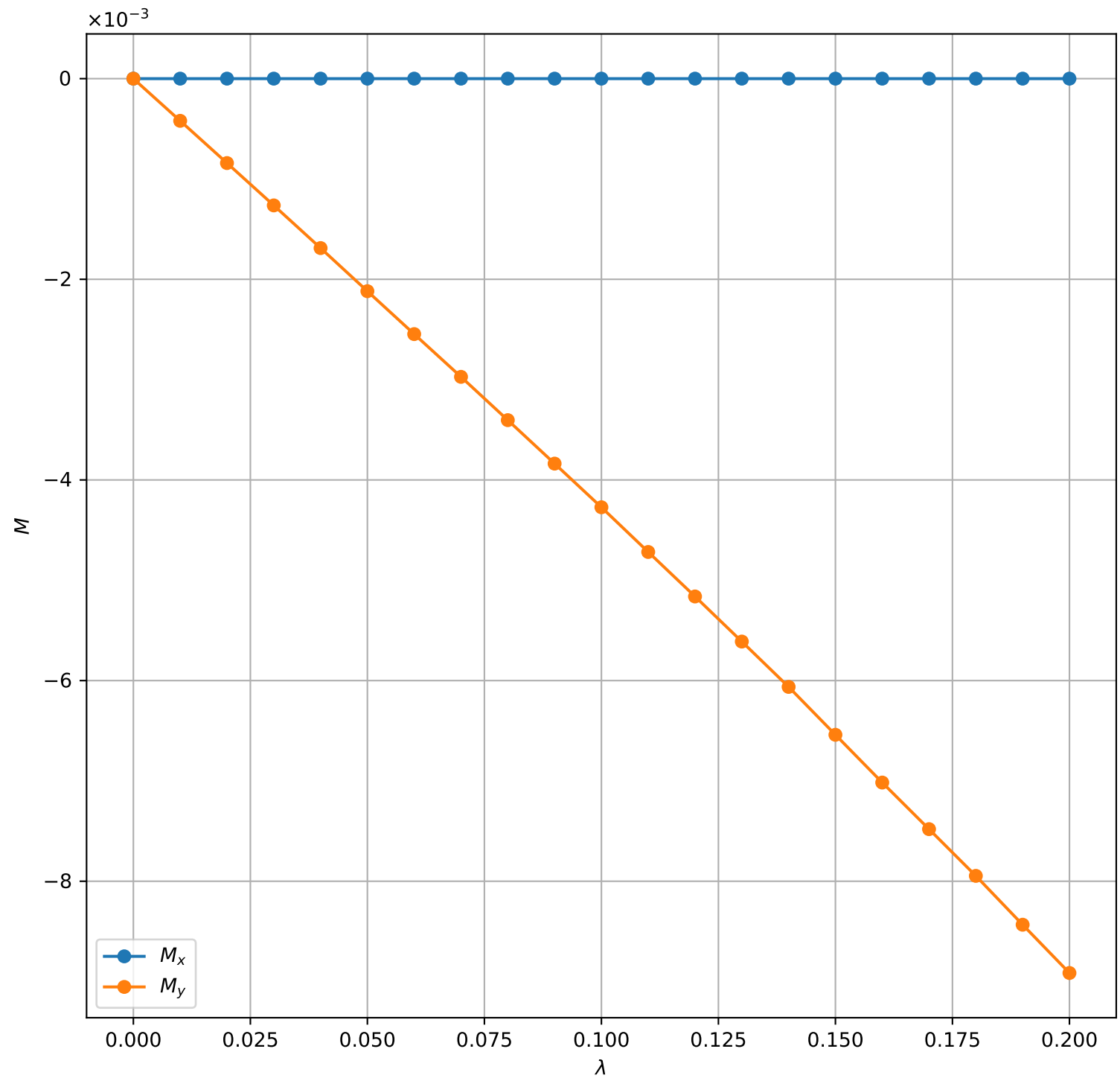
Bilayer QWZ Orbital Magnetization ( m = 1.0 , t_{\perp} = 0.2 , \mu = -1.0 , \delta = 1.00e-05 , N_k = 251 )
