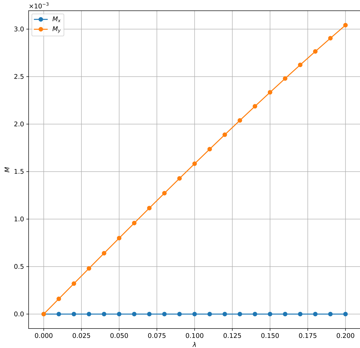
Bilayer QWZ Orbital Magnetization ( m = 1.0 , t_{\perp} = 0.2 , \mu = 0.0 , \delta = 1.00e - 05 , N_k = 251 )
