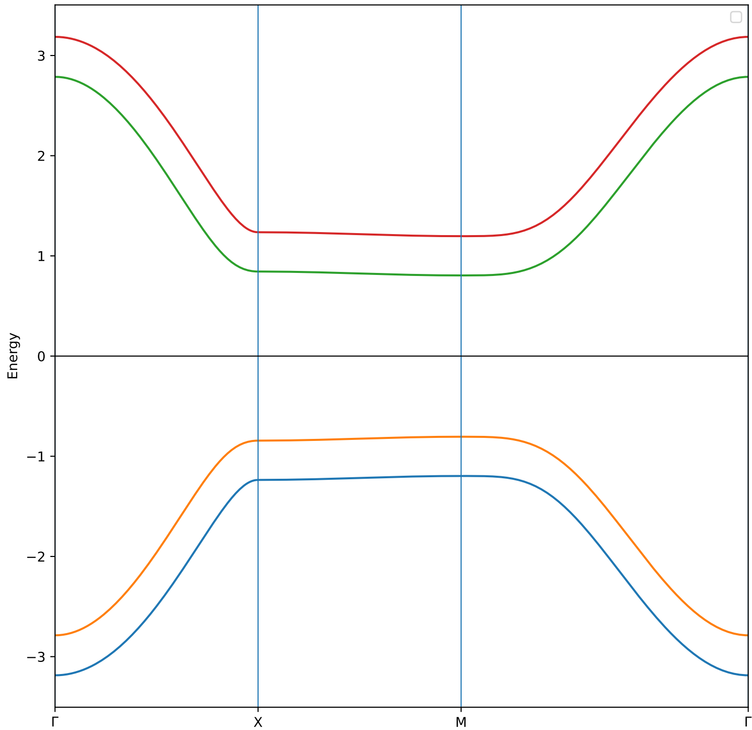
Bilayer QWZ band structure ( m = 1.0 , t_{\perp} = 0.2 , \lambda = 0.200 )
