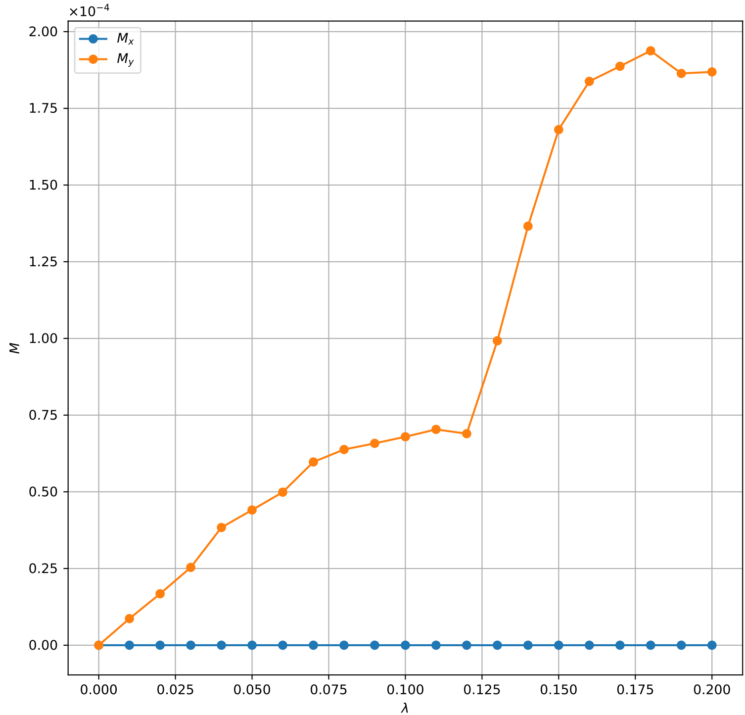
Bilayer QWZ Orbital Magnetization ( m = 1.0 , t_{\perp} = 0.2 , \mu = 1.5 , \delta = 1.00e - 03 , N_k = 101 )
