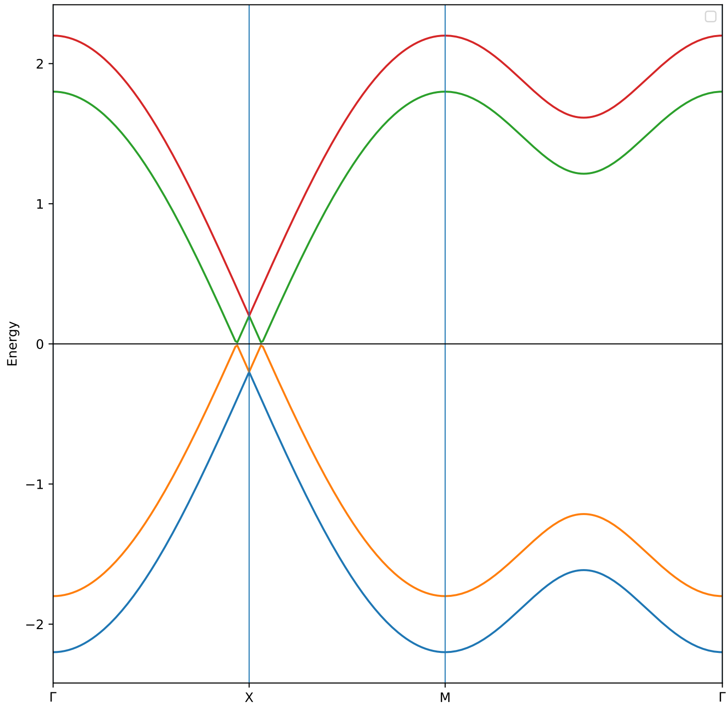
Bilayer QWZ band structure ( m = 0.0 , t_{\perp} = 0.2 , \lambda = 0.000 )
