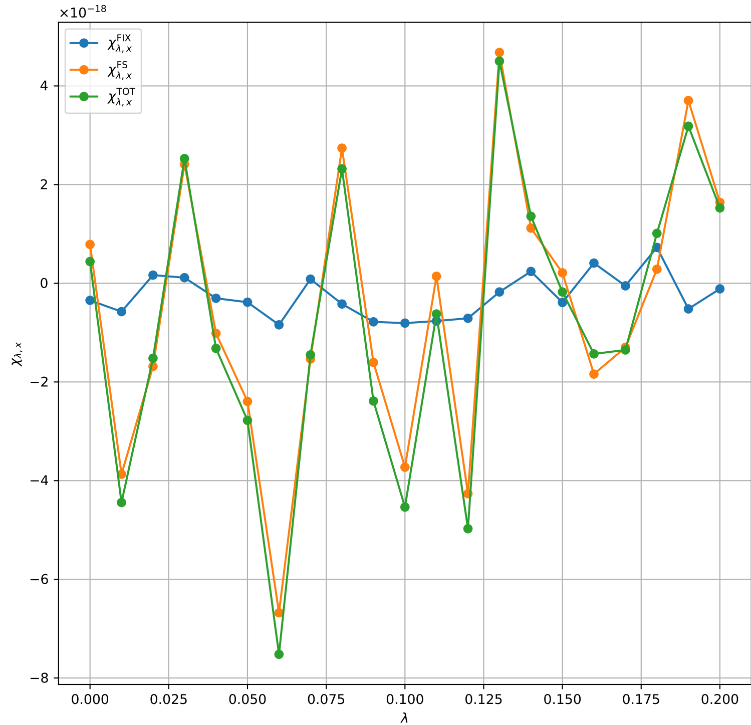
Bilayer QWZ Susceptibility ( m = 1.0 , t_{\perp} = 0.2 , \mu = -1.0 , \eta = 0.03 , N_k = 251 )
