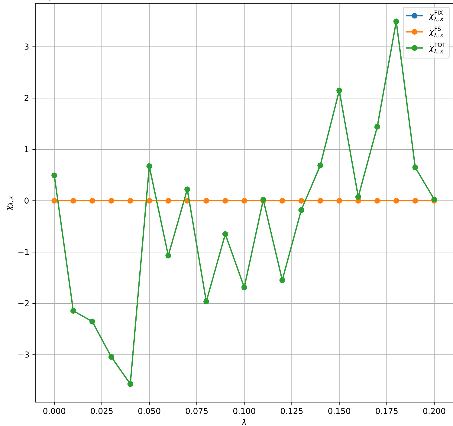
\times 10^{-19} Bilayer QWZ Susceptibility ( m = 1.0 , t_{\perp} = 0.2 , \mu = 0.0 , \eta = 0.03 , N_k = 251 )
