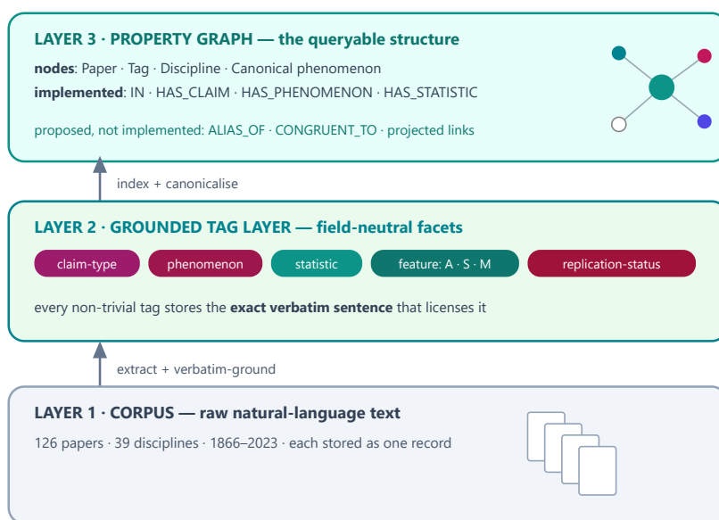
Fig. 1. The data structure: one property graph in three layers. A corpus of raw text (Layer 1) carries a grounded tag layer (Layer 2), which is read as a graph of nodes and edges (Layer 3) over which verification becomes a query. Full specification in the project's GRAPH_SCHEMA .
