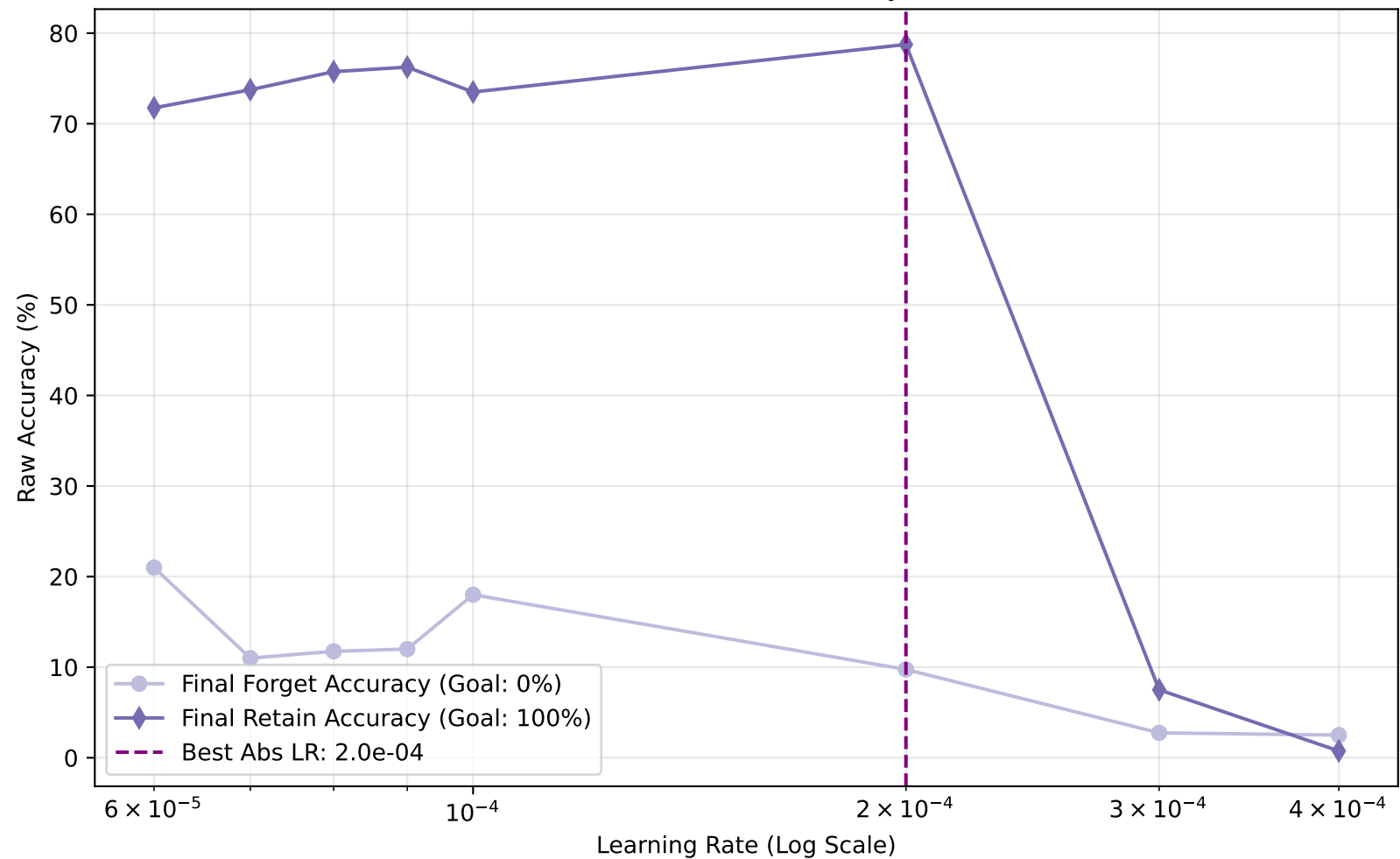
Option 2: Absolute Unlearning Performance (Final Model State Only)
