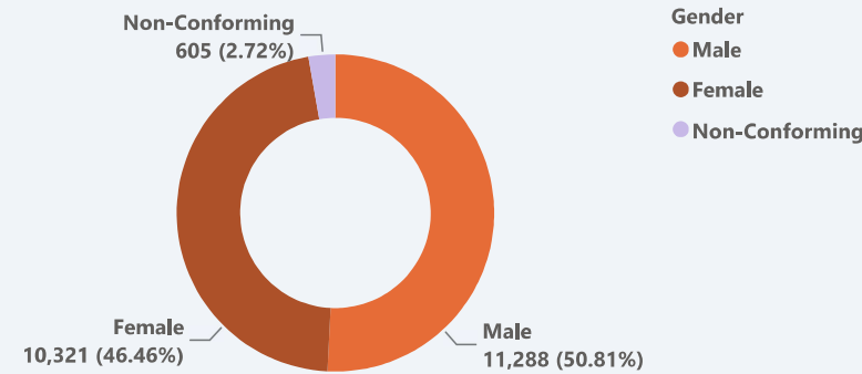
Gender Distribution
