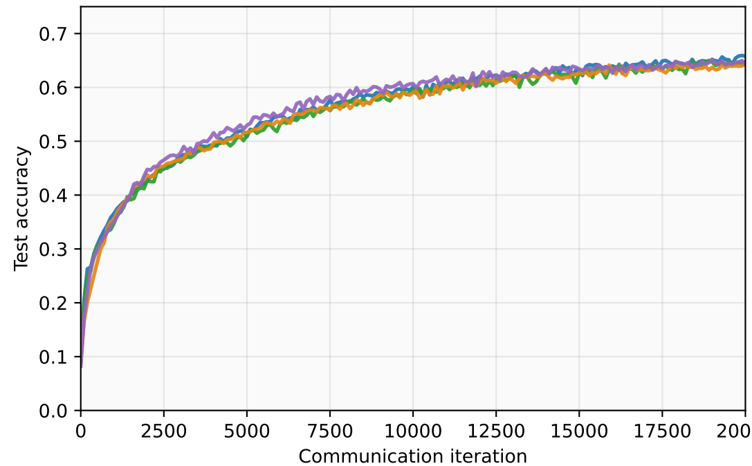
CIFAR-10 b=3 under HisMSA
