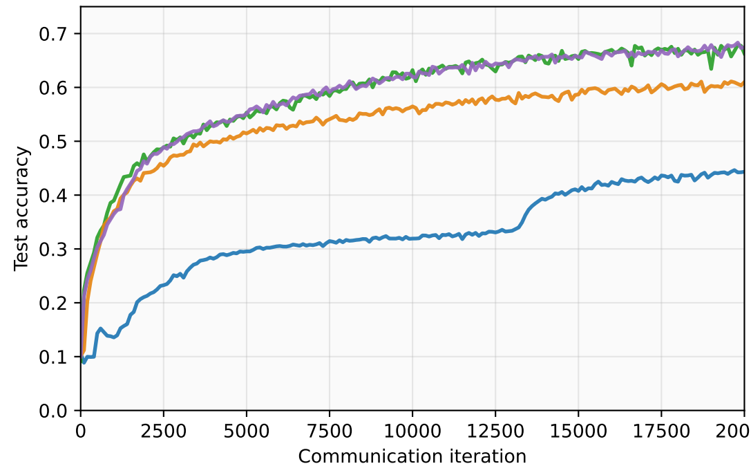
CIFAR-10 b=3 under MSA
