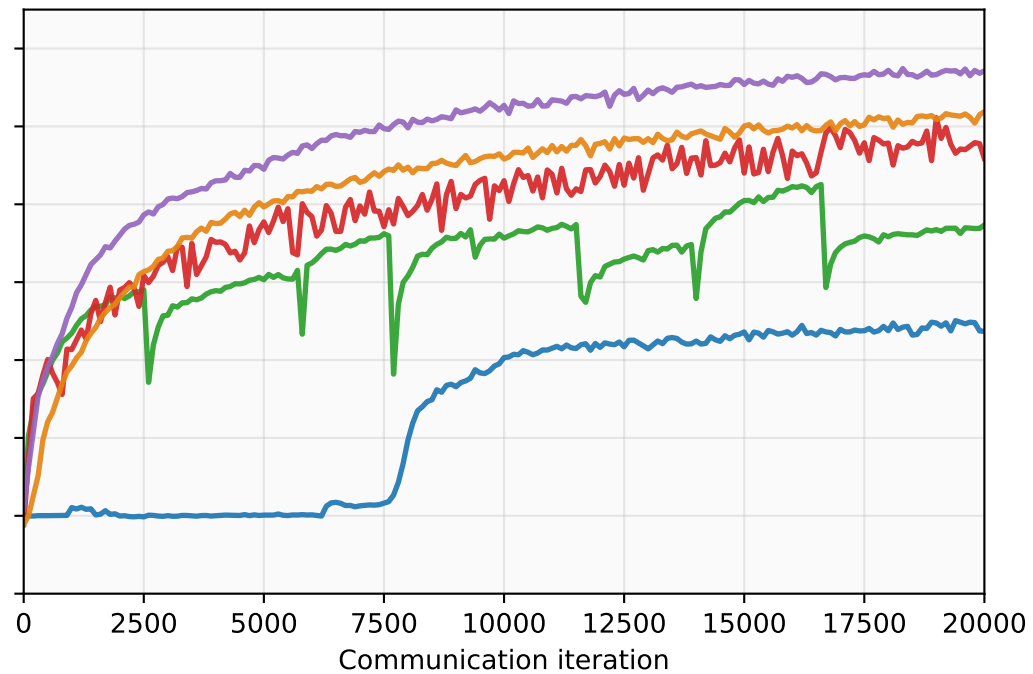
CIFAR-10 b=3 under MSA
