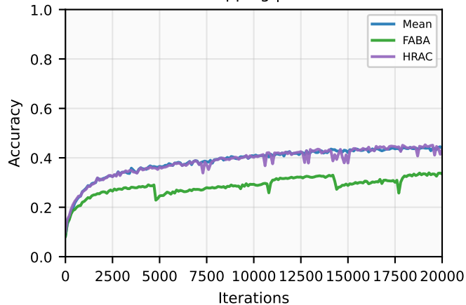
Label flipping | Non-IID
