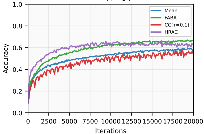
Label flipping | IID
