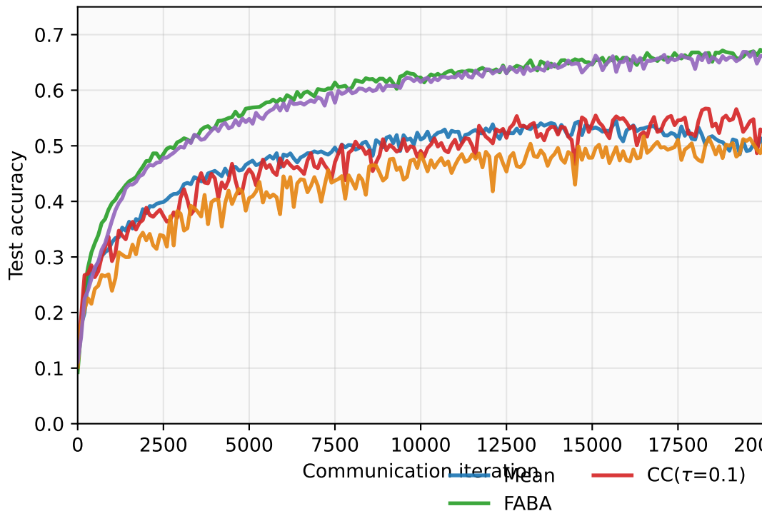
CIFAR-10 b=3 under Bit flipping
