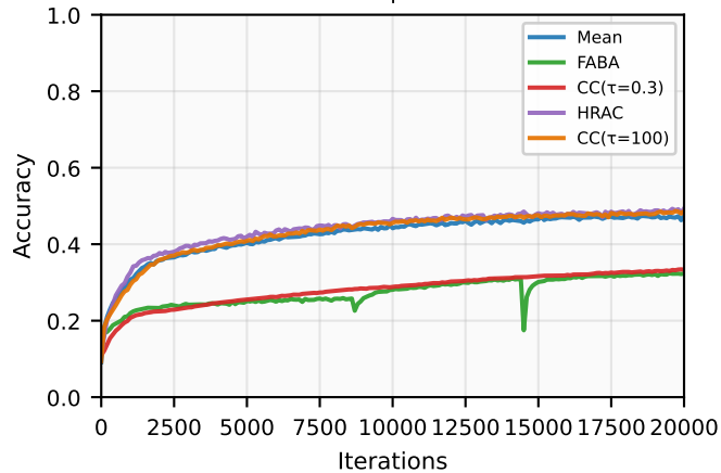
HisMSA | Non-IID
