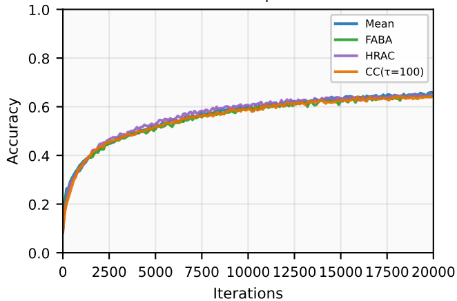
HisMSA | IID
