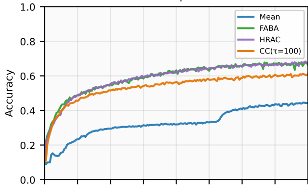
MSA | IID
