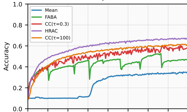
MSA | Non-IID
