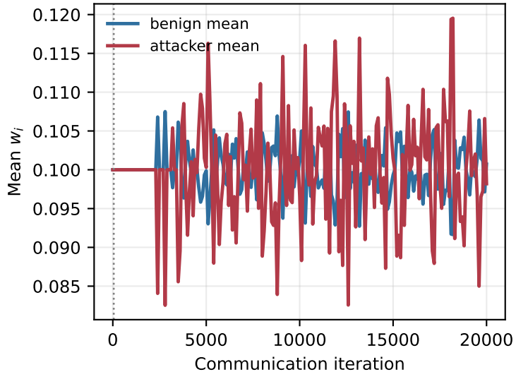
HRAC diagnostics on IID CIFAR-10 under MSA Normalised aggregation weight
