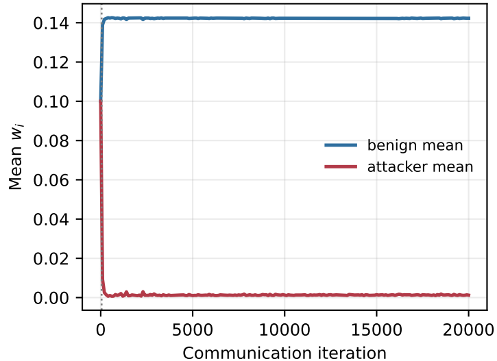
Normalised aggregation weight
