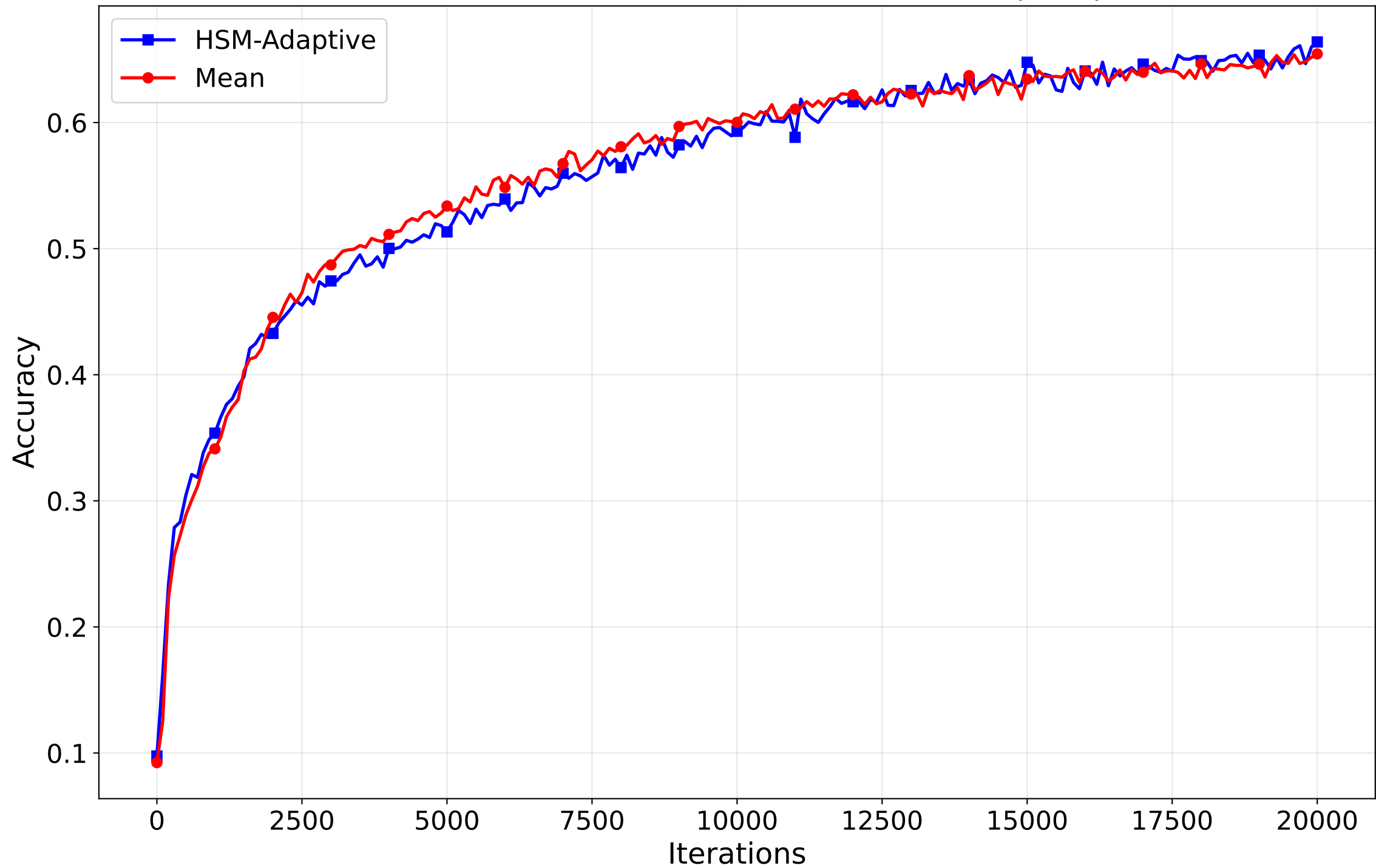
CIFAR-10 - IID Partition - HisMSA Attack (b=3)
