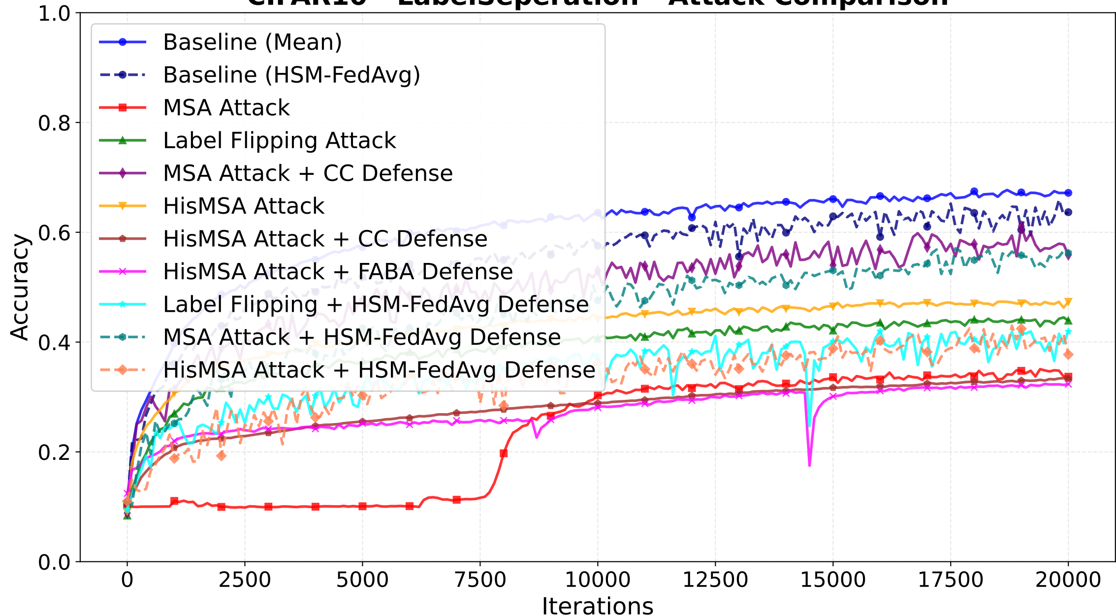
CIFAR10 - LabelSeperation - Attack Comparison
