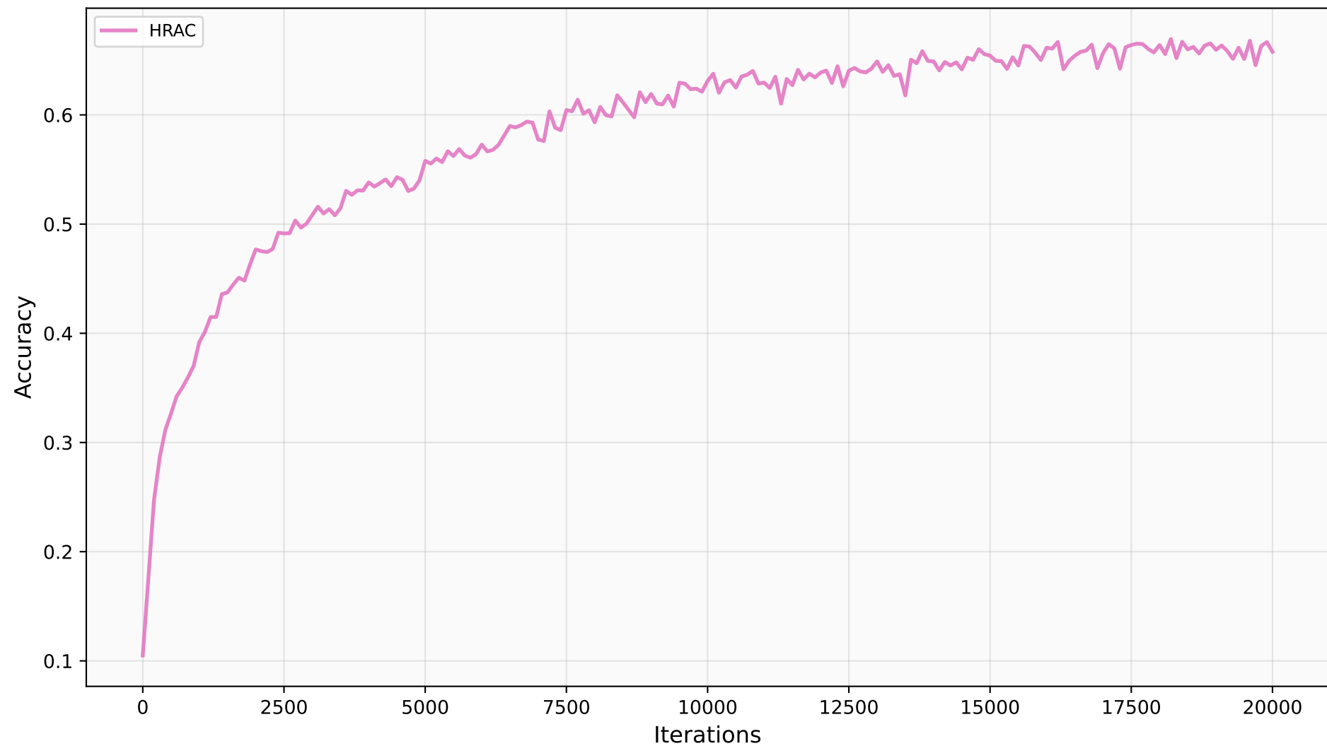
CIFAR10 b=3 — ALIE under IID
