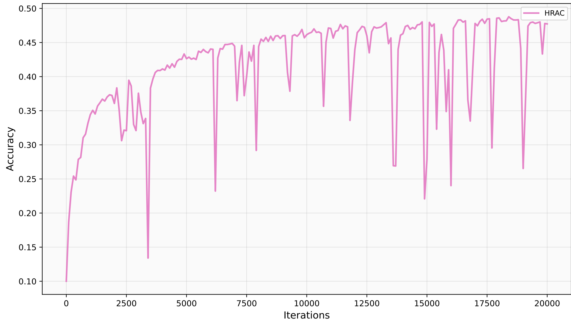
CIFAR10 b=3 — ALIE under Non-IID
