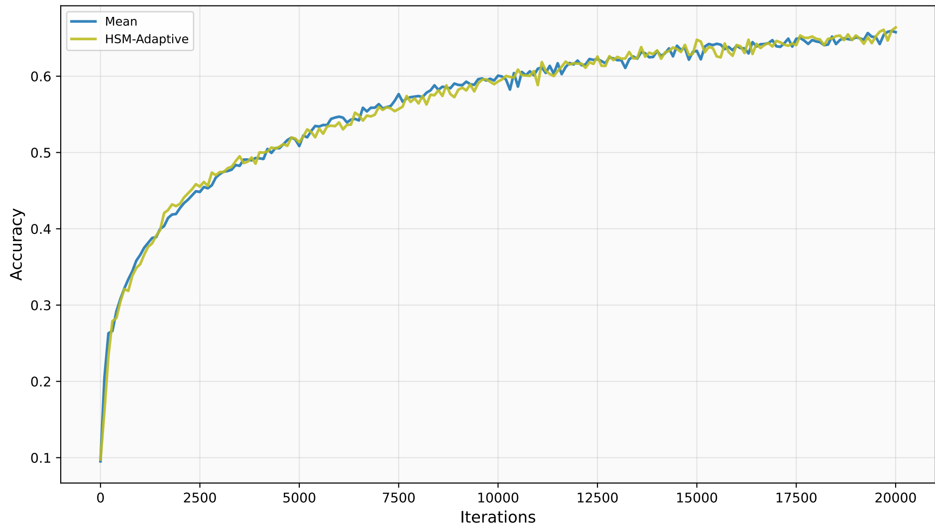
CIFAR10 b=3 — HisMSA under IID
