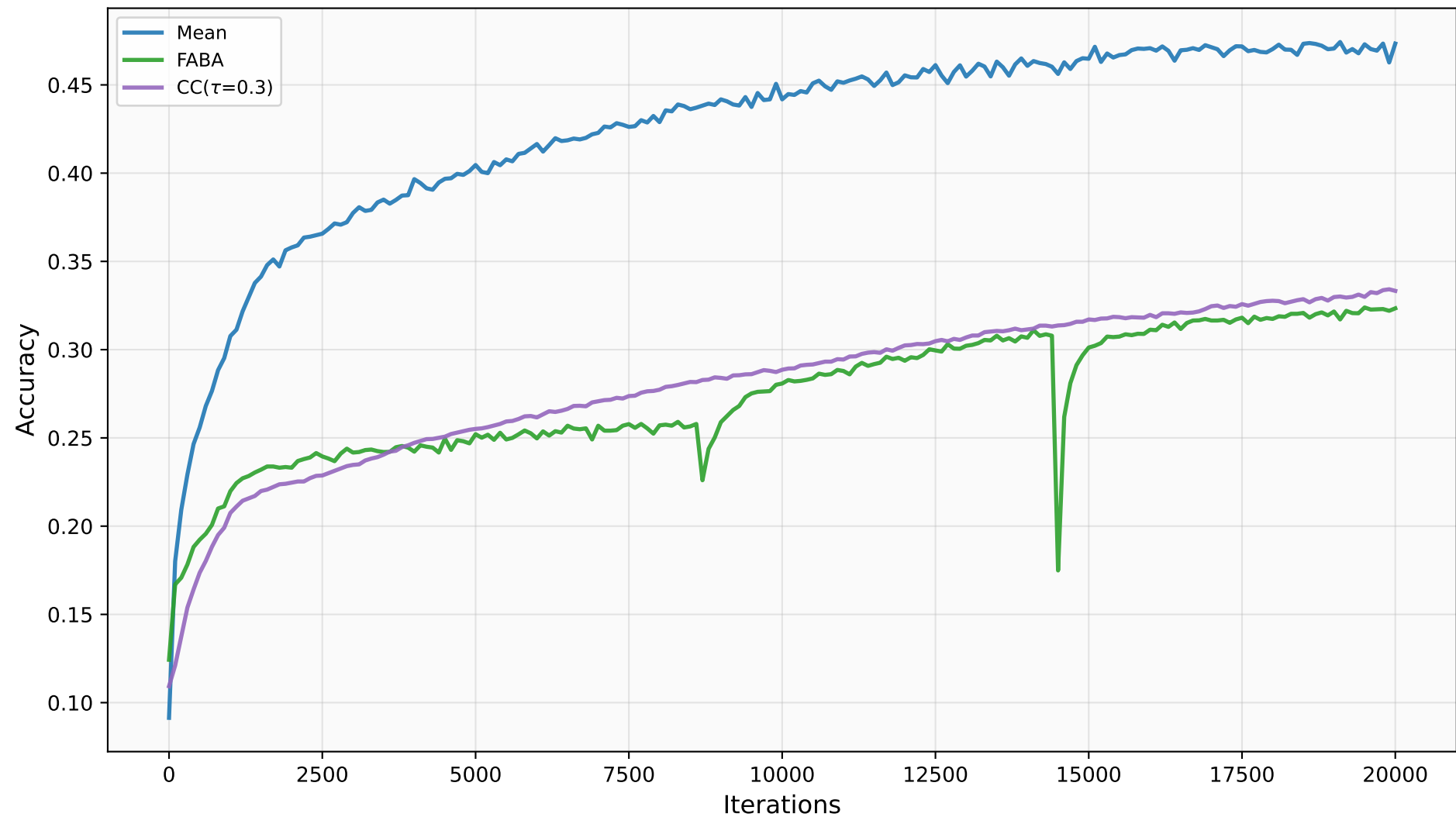
CIFAR10 b=3 — HisMSA under Non-IID
