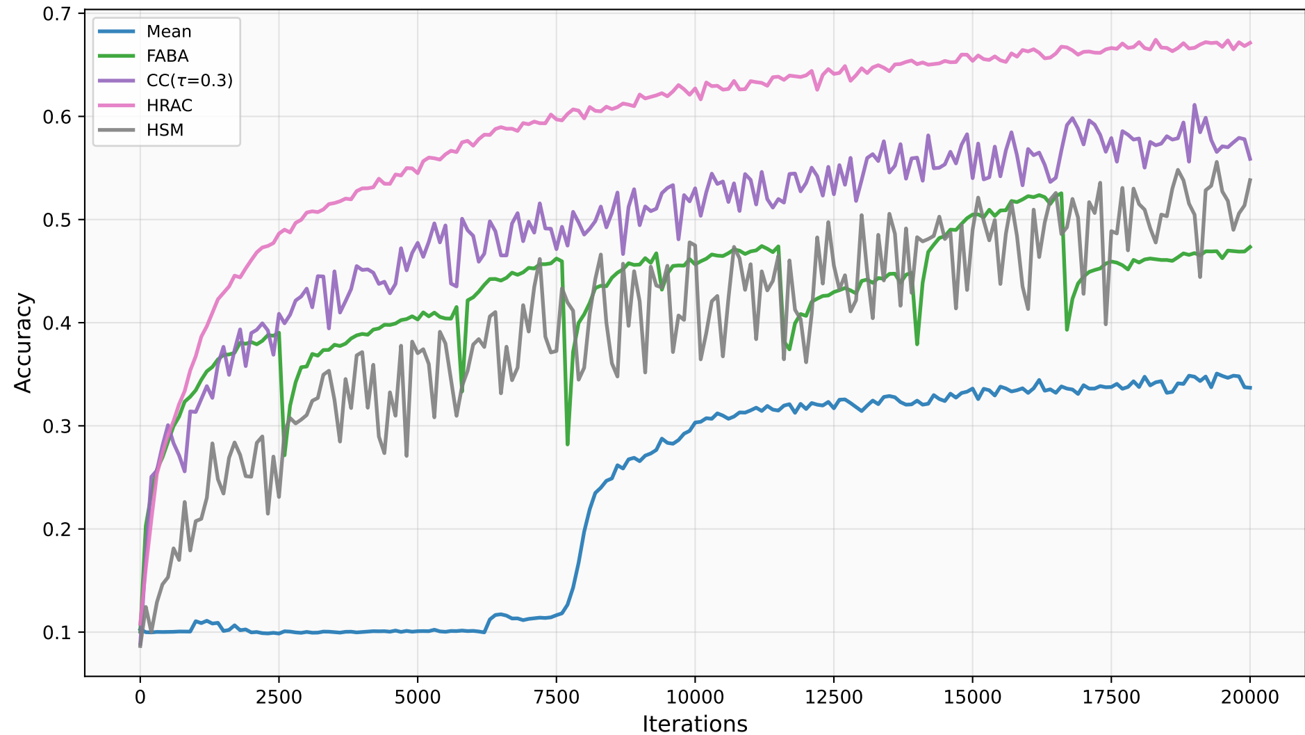
CIFAR10 b=3 — MSA under Non-IID
