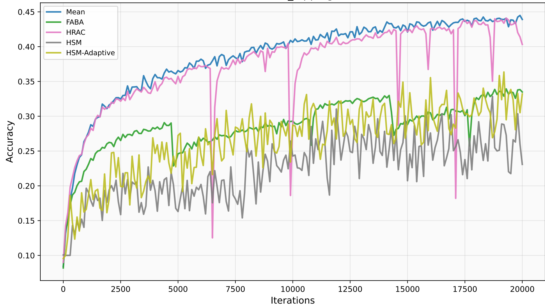
CIFAR10 b=3 — label_flipping under Non-IID
