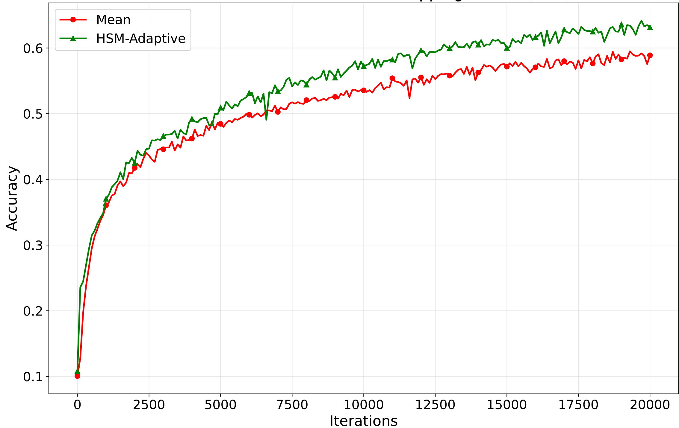
CIFAR-10 - IID Partition - Label Flipping Attack (b=3)
